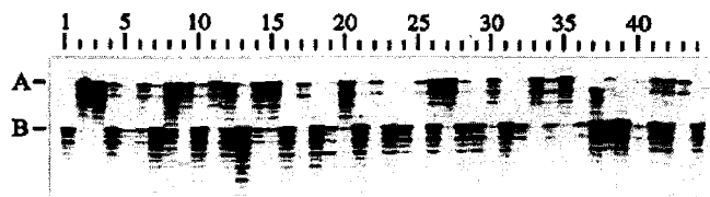
Figure 3. Autoradiograph showing the results of 50 genotyping experiments using the same extract (1:1) as template. Only the 44 positive amplifications are shown. Both alleles A and B are represented in the experiments of lanes 4–8, 10, 12–15, 19, 21, 26, 28, 30, 32, 34, 38 and 40–42. Only one allele, A or B, is represented in the experiments of lanes 1–3, 9, 11, 16–18, 20, 22–25, 27, 29, 31, 33, 35–37, 39, 43 and 44. Lanes 19 and 37 show two obvious false alleles. Lanes 3, 13, 20 and 34 may also contain false alleles.
